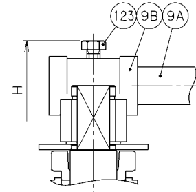
SIZE 150,200 Construction of LEVER HANDLE
