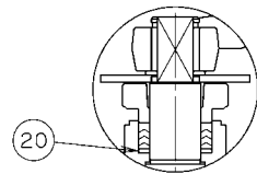
SIZE 15~32 Construction of GLAND PACKING
